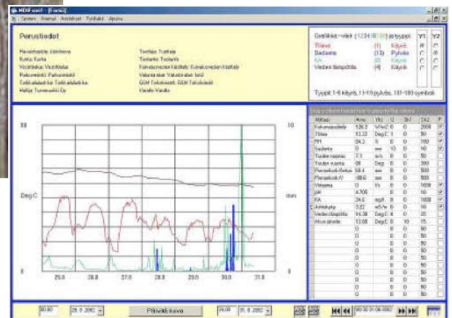
Continuous Monitoring of flow, pH and suspended material.
